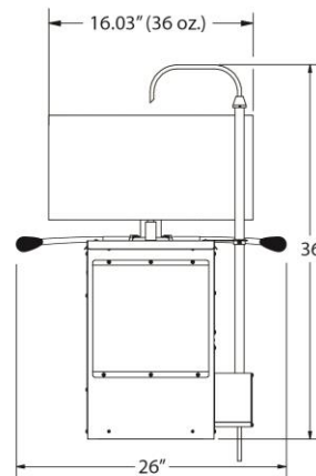
End View
