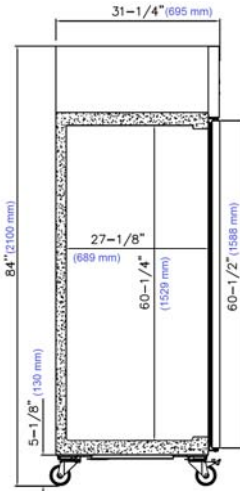
RIGHT VIEW
