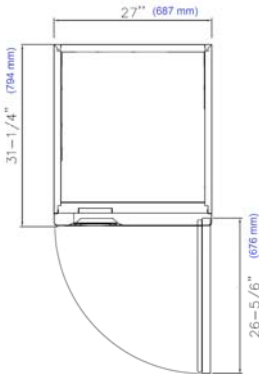
PLAN VIEW
