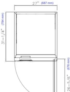
PLAN VIEW
