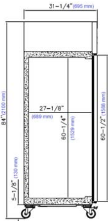
RIGHT VIEW
