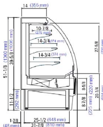
RIGHT VIEW
