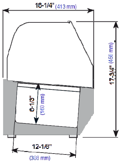
RIGHT VIEW
