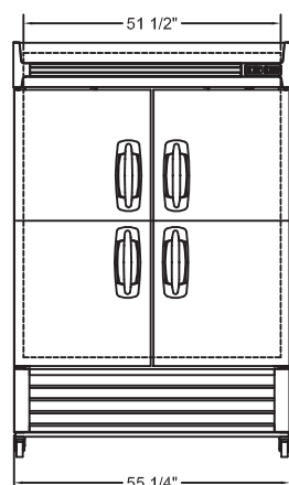
NLR49-SH FRONT
