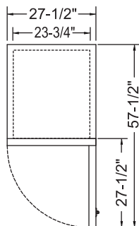
NLR23-SH TOP
