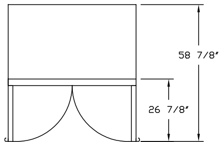
NR522 TOP VIEW
