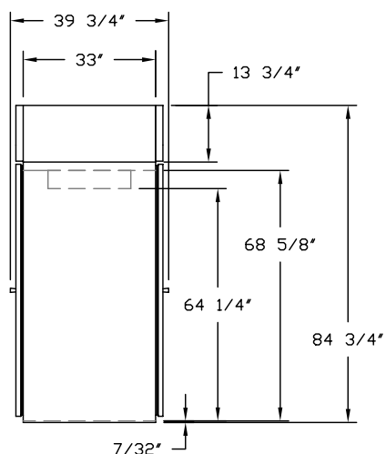
SIDE VIEW BOTH MODELS
