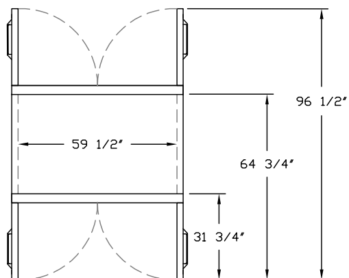
TOP VIEW PWW724
