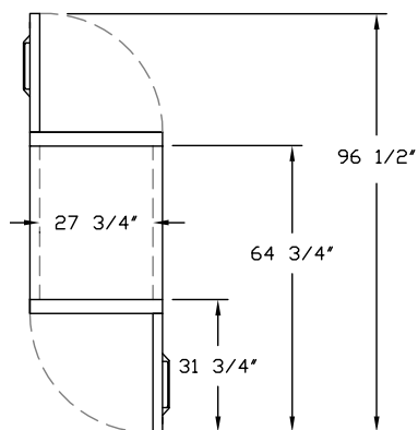
TOP VIEW PWW332
