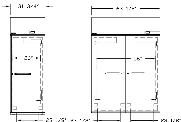
FRONT VIEW PWW332 PWW724
