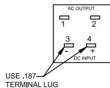
SSR PIN ASSIGNMENTS
